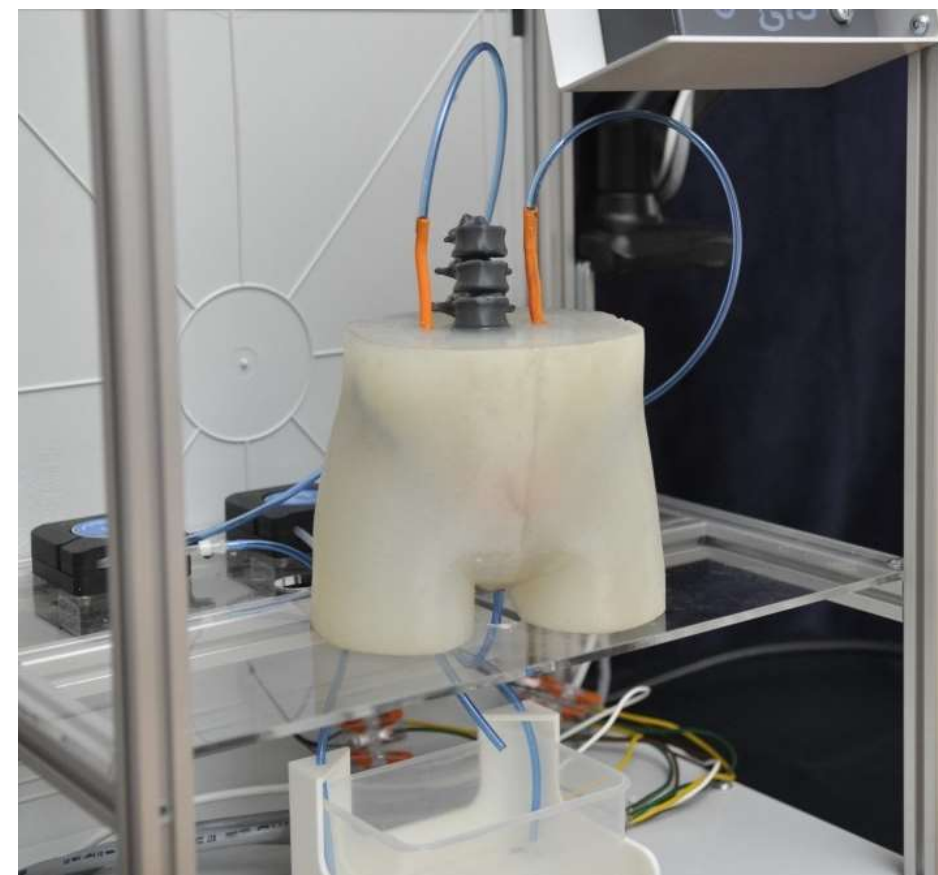
urology phantom
